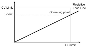
Power Supply I-V Diagram, CV Operation
