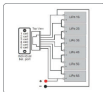
Balance wiring diagram
